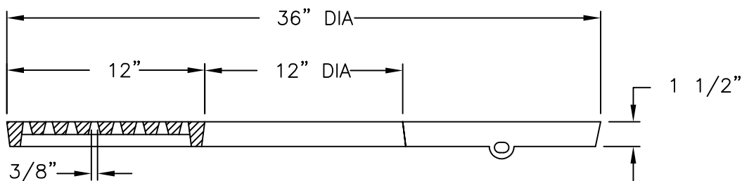
GRATE SECTION
